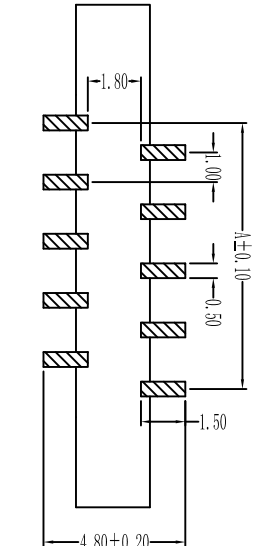
PCB Layout
